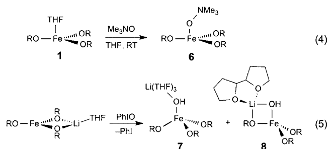
Figure 6. Reactivity of trigonal Fe(III) ditox compounds with oxo transfer reagents.
