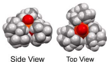
Figure 13. Space filling models of 9 depicting the accessibility of an apical oxygen atom (red) in a pseudo-tetrahedral geometry.
