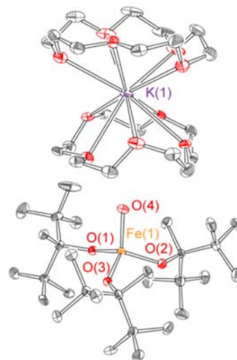
Figure 10. Structure [\text{Fe}(\text{ditox})_3(\text{OH})][\text{K}(\text{15C5})_2] , ( 9 ), 50% probability ellipsoids. H atoms are omitted for clarity. Selected bond distances: d(\text{Fe1}-\text{O1}) = 1.868(2) Å, d(\text{Fe1}-\text{O2}) = 1.859(1) Å, d(\text{Fe1}-\text{O3}) = 1.859(1) Å, d(\text{Fe1}-\text{O4}) = 1.890(1) Å. Selected bond angles: \angle(\text{O1}-\text{Fe1}-\text{O2}) = 108.0(1)^\circ , \angle(\text{O1}-\text{Fe1}-\text{O3}) = 111.1(1)^\circ , \angle(\text{O2}-\text{Fe1}-\text{O3}) = 109.2(1)^\circ , \angle(\text{O1}-\text{Fe1}-\text{O4}) = 110.0(0)^\circ , \angle(\text{O2}-\text{Fe1}-\text{O4}) = 111.4(1)^\circ , \angle(\text{O3}-\text{Fe1}-\text{O4}) = 107.2(2)^\circ .
