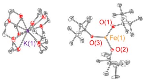
Figure 5. Structure of [\text{Fe}(\text{ditox})_3][\text{K}(15\text{C}5)_2] , ( 5 ), 50% probability ellipsoids. Hydrogen atoms omitted for clarity. Selected bond distances: d(\text{Fe1}-\text{O1}) = 1.864(2) Å, d(\text{Fe1}-\text{O2}) = 1.870(2) Å, d(\text{Fe1}-\text{O3}) = 1.865(2) Å. Selected bond angles: \angle(\text{O1}-\text{Fe1}-\text{O2}) = 120.2(1)^\circ , \angle(\text{O1}-\text{Fe1}-\text{O3}) = 120.1(1)^\circ , \angle(\text{O2}-\text{Fe1}-\text{O3}) = 119.6(1)^\circ .
