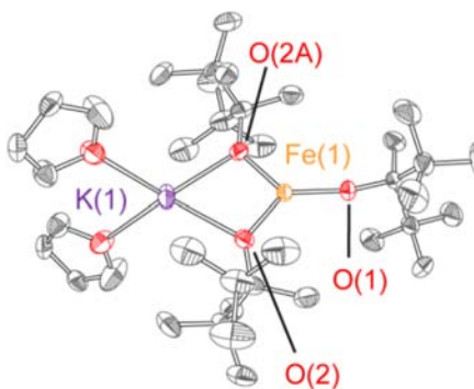
Figure 4. Structure of \text{Fe}(\text{ditox})_3\text{K}(\text{THF})_2 ( 4 ), 50% probability ellipsoids. H atoms are omitted for clarity. Selected bond distances: d(\text{Fe1}-\text{O1}) = 1.826(2) \text{ \AA} , d(\text{Fe1}-\text{O2}) = 1.903(1) \text{ \AA} , d(\text{K1}-\text{O2}) = 2.585(1) \text{ \AA} . Selected bond angles: \angle(\text{O1}-\text{Fe1}-\text{O2}) = 130.1(1)^\circ , \angle(\text{K1}-\text{O2}-\text{Fe1}) = 95.8(1)^\circ , \angle(\text{O2}-\text{Fe1}-\text{O2A}) = 99.8(1)^\circ .
