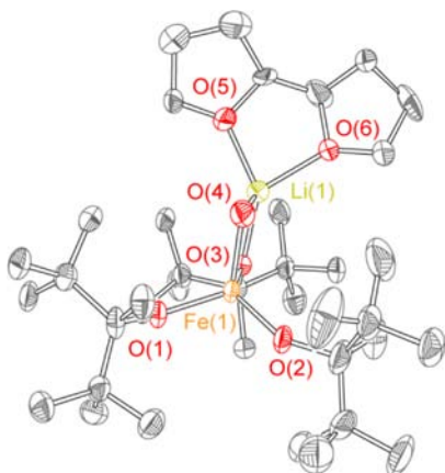
Figure 8. Structure of \text{Fe}(\text{ditox})_3(\text{OH})\text{Li}(\text{C}_8\text{O}_2\text{H}_{14}) , ( 8 ), 50% probability. H atoms and alternative conformations of t Bu groups are omitted for clarity. Selected bond distance: d(\text{Fe1}-\text{O1}) = 1.836(2) Å, d(\text{Fe1}-\text{O2}) = 1.823(2) Å, d(\text{Fe1}-\text{O3}) = 1.919(2) Å, d(\text{Fe1}-\text{O4}) = 1.920(2) Å, d(\text{Li1}-\text{O3}) = 1.949(5) Å, d(\text{Li1}-\text{O4}) = 1.885(7) Å, d(\text{Li1}-\text{O5}) = 1.995(5) Å, d(\text{Li1}-\text{O6}) = 2.014(5) Å. Selected bond angles: \angle(\text{O1}-\text{Fe1}-\text{O2}) = 111.4(1)^\circ , \angle(\text{O1}-\text{Fe1}-\text{O3}) = 111.5(1)^\circ , \angle(\text{O2}-\text{Fe1}-\text{O3}) = 121.8(1)^\circ , \angle(\text{O1}-\text{Fe1}-\text{O4}) = 111.4(1)^\circ , \angle(\text{O2}-\text{Fe1}-\text{O4}) = 110.6(1)^\circ , \angle(\text{O3}-\text{Fe1}-\text{O4}) = 87.9(1)^\circ , \angle(\text{O3}-\text{Li1}-\text{O4}) = 88.0(2)^\circ . The analogous structure with uncoupled THF molecules, 7a , is shown in the Supporting Information, Figure S2.
