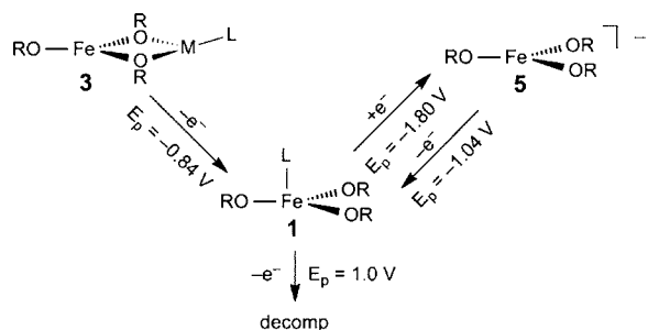
Scheme 1. Electrochemical Behavior of Fe Ditox Complexes
