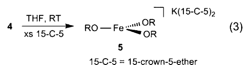
Figure 1. Preparative reactions of Fe ditox compounds.
