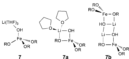
Figure 9. Solvation state differences for \text{Fe}(\text{ditox})_3(\text{OH})\text{Li} .
