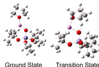
Figure 12. Optimized structures for the ground state geometry of \text{Fe}(\text{O}^t\text{Bu})_3(\text{O})\text{Li}(\text{THF}) and the corresponding transition state for hydrogen atom abstraction from \alpha carbon of the coordinated THF.
