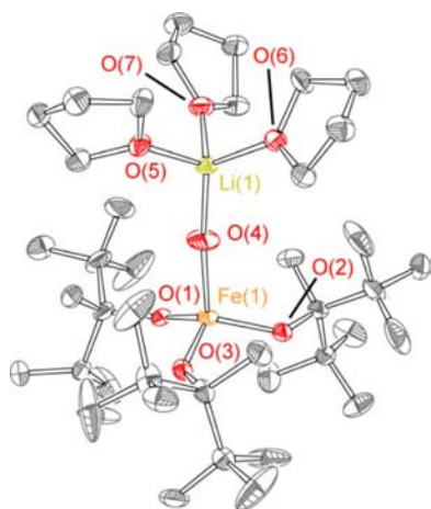
Figure 7. Structure of \text{Fe}(\text{ditox})_3(\text{OH})\text{Li}(\text{THF})_3 , ( 7 ), 30% probability ellipsoids. H atoms, co-crystallized solvent molecules, and alternative conformations of t Bu groups are omitted for clarity. Selected bond distances: d(\text{Fe1}-\text{O1}) = 1.842(5) Å, d(\text{Fe1}-\text{O2}) = 1.860(4) Å, d(\text{Fe1}-\text{O3}) = 1.850(5) Å, d(\text{Fe1}-\text{O4}) = 1.945(5) Å, d(\text{Li1}-\text{O4}) = 1.794(11) Å. Selected bond angles: \angle(\text{O1}-\text{Fe1}-\text{O2}) = 111.2(2)^\circ , \angle(\text{O1}-\text{Fe1}-\text{O3}) = 111.4(2)^\circ , \angle(\text{O2}-\text{Fe1}-\text{O3}) = 110.9(2)^\circ , \angle(\text{O1}-\text{Fe1}-\text{O4}) = 107.4(3)^\circ , \angle(\text{O2}-\text{Fe1}-\text{O4}) = 109.5(2)^\circ , \angle(\text{O3}-\text{Fe1}-\text{O4}) = 106.3(3)^\circ , \angle(\text{Fe1}-\text{O4}-\text{Li1}) = 173.5(6)^\circ .
