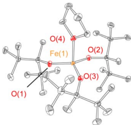
Figure 2. Structure of \text{Fe}(\text{ditox})_3\text{THF} ( 1 ), 50% probability ellipsoids. H atoms are omitted for clarity. Selected bond distances: d(\text{Fe1}-\text{O1}) = 1.822(2) \text{ \AA} , d(\text{Fe1}-\text{O2}) = 1.823(2) \text{ \AA} , d(\text{Fe1}-\text{O3}) = 1.826(2) \text{ \AA} , d(\text{Fe1}-\text{O4}) = 2.089(2) \text{ \AA} . Selected bond angles: \angle(\text{O1}-\text{Fe1}-\text{O2}) = 113.4(1)^\circ , \angle(\text{O1}-\text{Fe1}-\text{O3}) = 119.8(1)^\circ , \angle(\text{O2}-\text{Fe1}-\text{O3}) = 118.8(1)^\circ , \angle(\text{O1}-\text{Fe1}-\text{O4}) = 102.4(1)^\circ , \angle(\text{O2}-\text{Fe1}-\text{O4}) = 101.1(1)^\circ , \angle(\text{O3}-\text{Fe1}-\text{O4}) = 95.0(1)^\circ .
